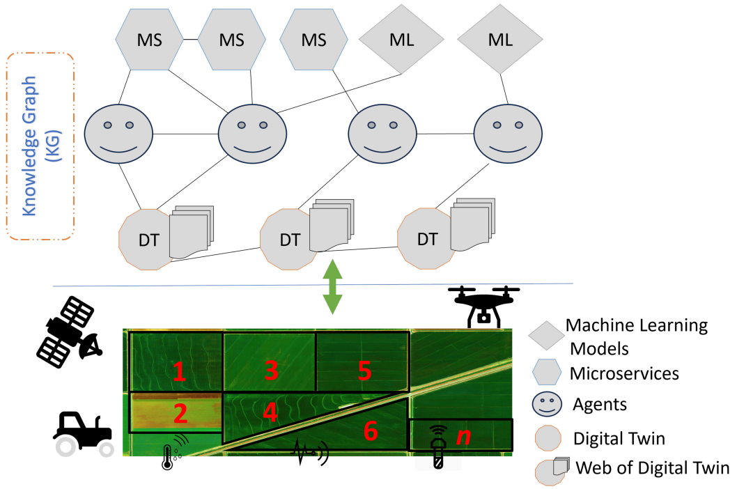
Fig. 2. Proposed architecture for a digital twin in open-environment arable farming.
